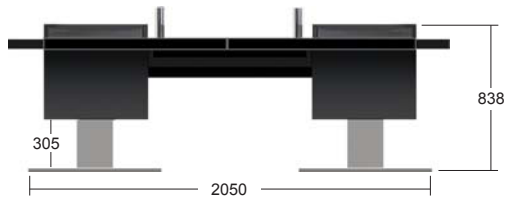
Mirage DC8 Dimensions
