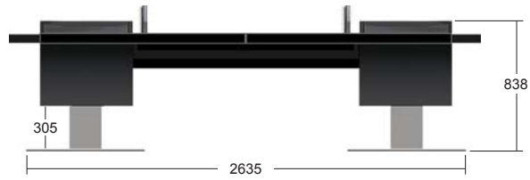
Mirage DC24 Dimensions
