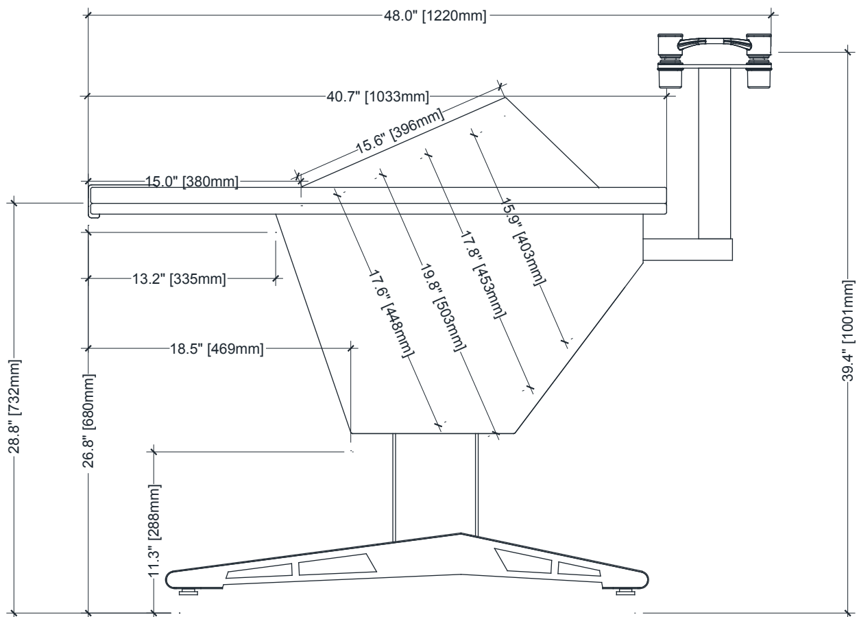
Side View Showing Rack
