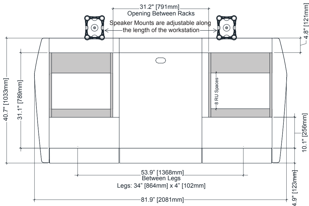
Eclipse Universal Workstation 682mm Desk Space
