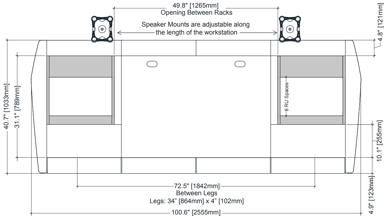
Eclipse Universal Workstation 1156mm Desk Space
